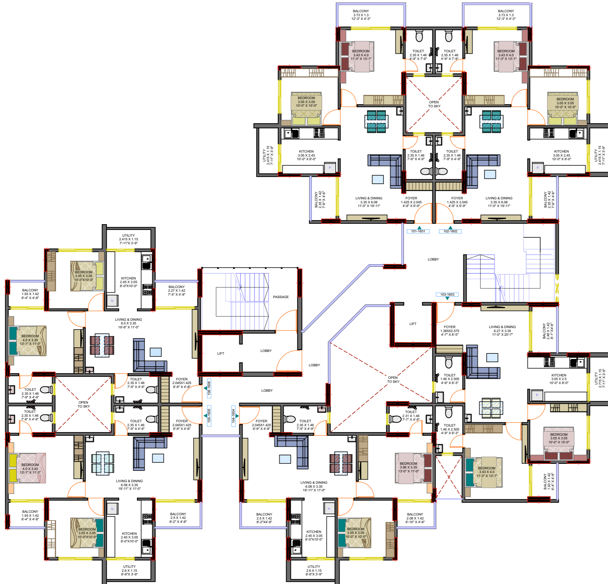
WING A - TYPICAL FLOOR 1ST TO 7TH, 9TH TO 12TH & 14TH TO 16TH
