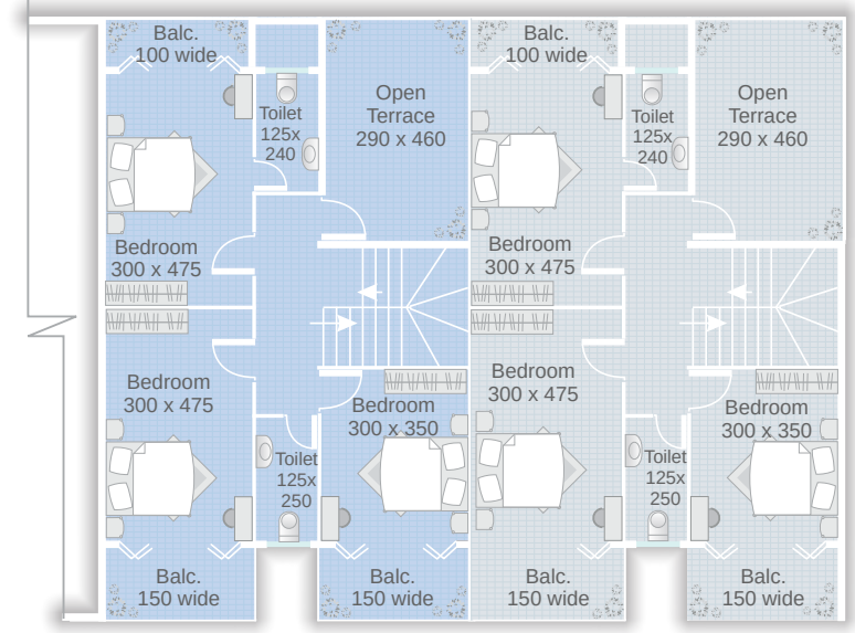
FIRST FLOOR PLAN TYPE B
