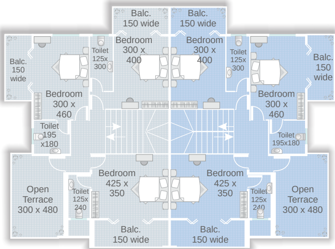
FIRST FLOOR PLAN TYPE A1 & A2
