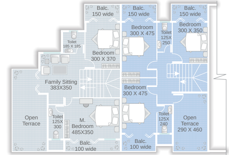
FIRST FLOOR PLAN TYPE BC
